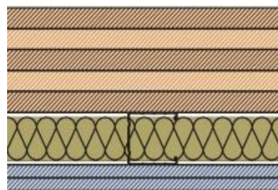
XLAM sp. 90mm + MONTANTE 50 Geo B-040 sp. 40mm 2 SUPER 13
