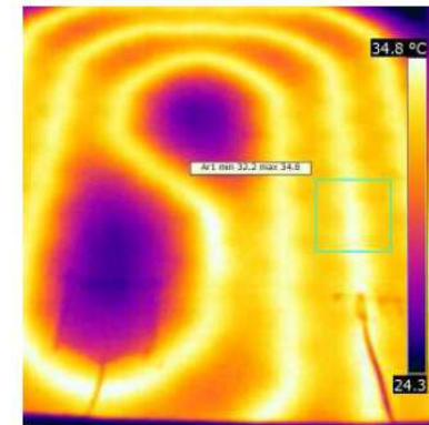
Ore 12:05 - NE499 Temperatura media area = 33,3°C
