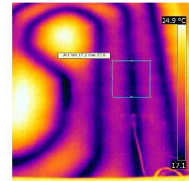
Ore 15:15 - NE499 Temperatura media area = 18,8°C
